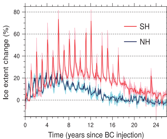
Figure 5. Change in sea ice extent (%) for the 50 nm experiment is shown relative to the control. Sea ice extent is defined as the area of all sea surface grid points with ice fraction greater than 15%. The red line shows the ensemble average anomaly for the Southern Hemisphere. The blue line shows the same for the Northern Hemisphere. Shading around each line shows the range of the experiment ensemble runs with respect to the control ensemble average. The horizontal axis shows time in years. The vertical axis shows relative change in ice extent area, 100\% \times (\text{experiment} - \text{control})/\text{control} .
