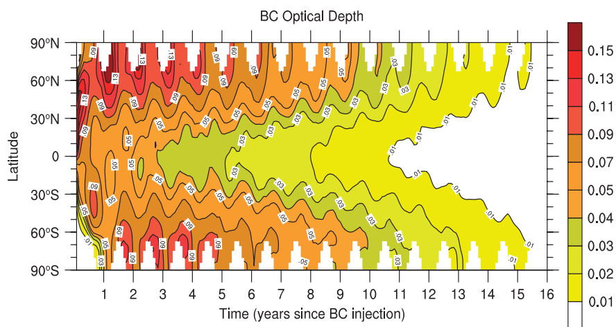
Figure 2. The time evolution of zonal mean total column BC optical depth in the visible part of the spectrum is shown for the 50 nm experiment ensemble average. The vertical axis shows latitude. The horizontal axis shows time in years.
