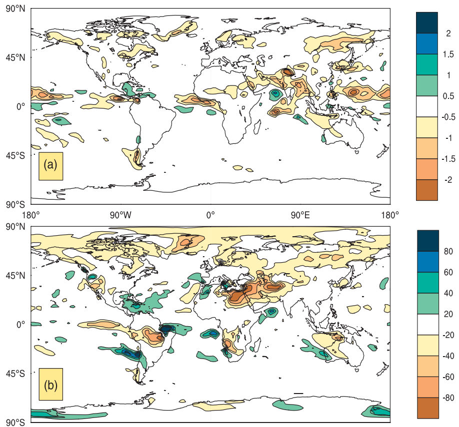
Figure 11. Changes in (a) absolute (mm/day) and (b) relative (%) surface precipitation. Values are 5 year seasonal ensemble averages for June to August, years 2–6, experiment minus control.
