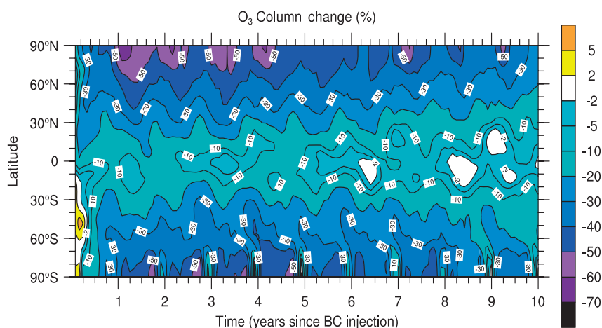
Figure 8. The time evolution of the change (%) in zonal mean column ozone is shown. The change in the 50 nm experiment ensemble average is shown relative to the control ensemble average: 100\% \times (\text{experiment} - \text{control})/\text{control} . The horizontal axis shows time in years. The vertical axis shows latitude.
