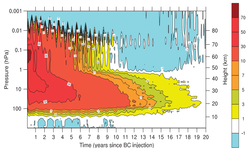
Figure 7. The time evolution of the vertical profile of global average temperature anomaly is shown. Values are for the 50 nm experiment ensemble average minus the control ensemble average. The horizontal axis shows time in years. The left vertical axis shows pressure in hPa, and the right vertical axis shows approximate pressure altitude in km. Contours show temperature anomalies in K.
