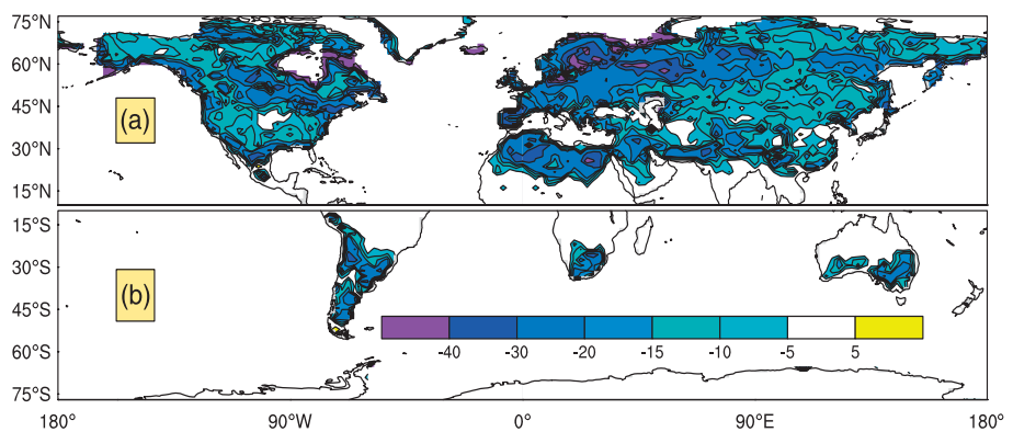
Figure 12. Change in frost-free growing season in days for (a) January to December in the Northern Hemisphere and (b) July to June in the Southern Hemisphere. Values are 5 year seasonal ensemble averages for years 2–6, experiment minus control.
