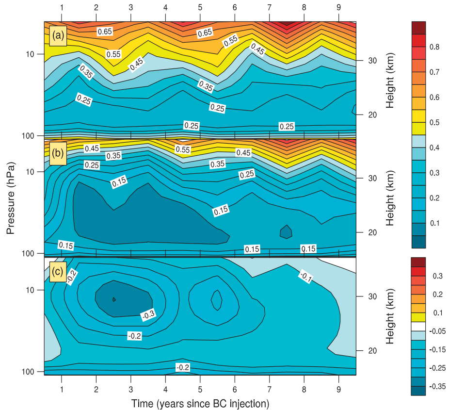
Figure 4. The time evolution of the tropical lower stratospheric vertical wind (mm/s) is shown for (a) the control, (b) the 50 nm experiment, and (c) the experiment minus the control. Values are ensemble averages for latitudes 22°S to 22°N. The horizontal axis shows time in years. The left vertical axis shows pressure in hPa, and the right shows approximate pressure altitude in km.
