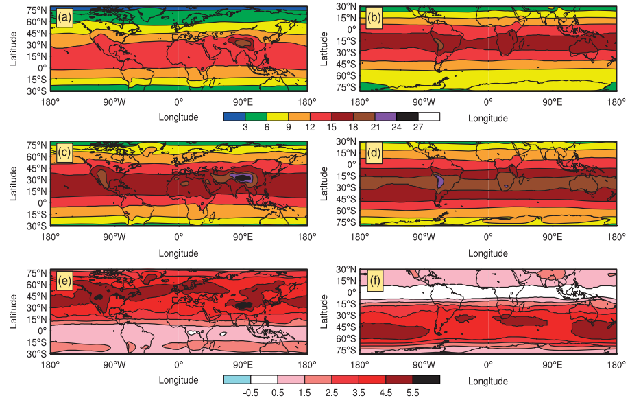
Figure 9. UV index in June (left) and December (right) is shown for the control (a, b), the experiment (c, d), and the experiment minus the control (e, f). Values are ensemble averages for year 3.
