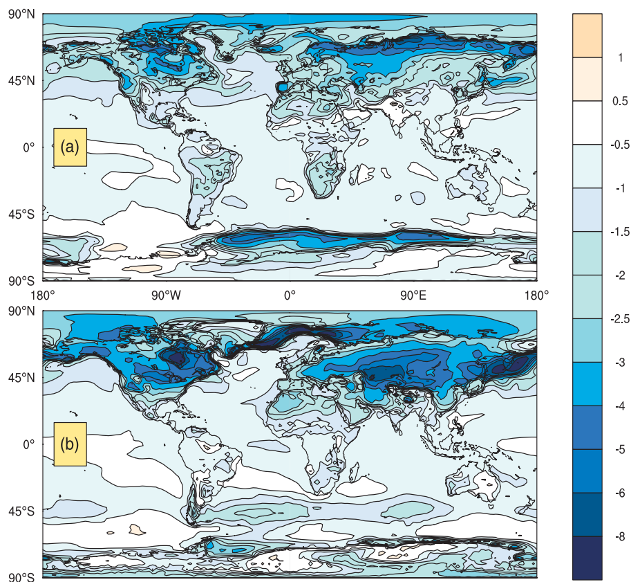
Figure 10. Change in surface temperature (K) for (a) June to August and (b) December to February. Values are 5 year seasonal ensemble averages for years 2–6, experiment minus control.
