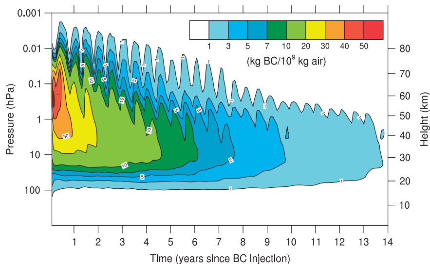
Figure 1. The time evolution of BC mass mixing ratio ( \text{kg BC}/10^9 \text{ kg air} ) is shown for the average of the 50 nm experiment ensemble. The horizontal axis shows time in years since the emission of 5 Tg BC at 150–300 hPa on 1 January.
