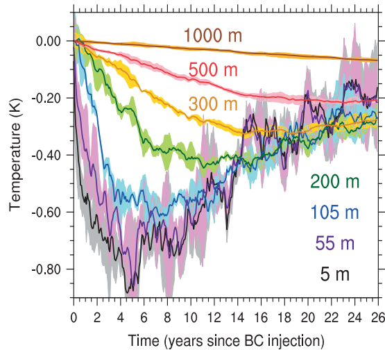
Figure 6. The time evolution of the global average ocean temperature anomaly at various depths is shown. The lines show the monthly average of the experiment ensemble temperatures minus the monthly average of the control ensemble. Shading around each line shows the range of the experiment ensemble runs with respect to the control ensemble average. The horizontal axis shows time in years. The vertical axis shows temperature in K.
