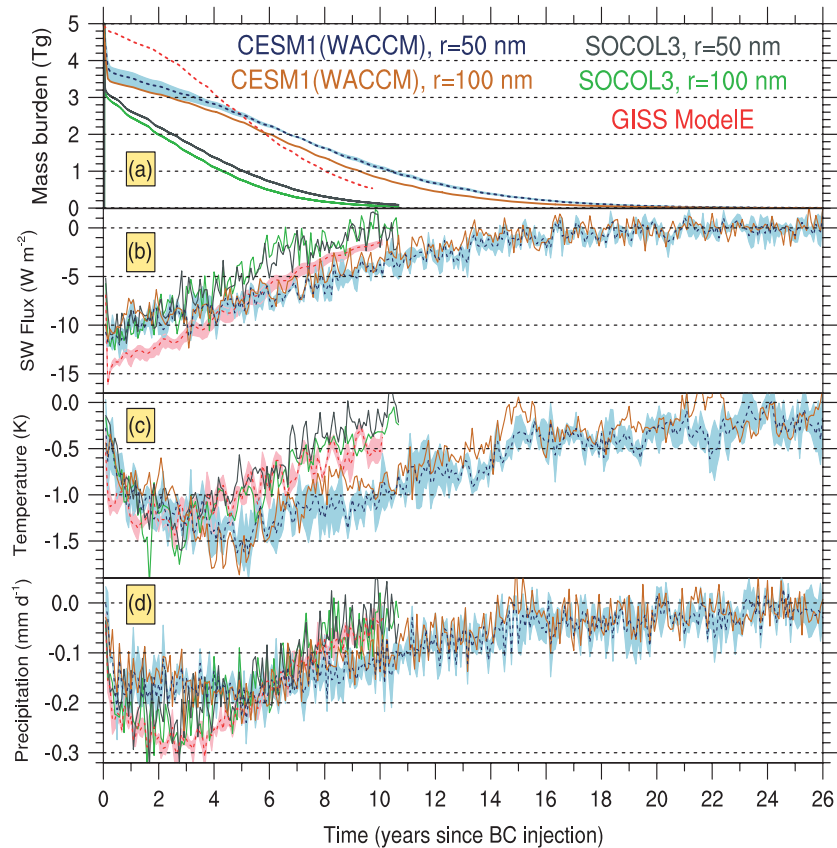
Figure 3. The monthly global mean time evolution is shown for (a) the mass burden of black carbon (Tg), (b) the shortwave net flux anomaly at the surface ( \text{W m}^{-2} ), (c) the surface temperature anomaly (K), and (d) the precipitation anomaly ( \text{mm/day} ). The dark blue dashed line and light blue shading show the average and range of our 50 nm experiment ensemble. The dark red dashed line and pink shading show the ensemble average and range for Rocco et al. [2007a, 2007b] (data courtesy L. Oman). The grey and green lines show results from two 5 Tg BC simulations from Stenke et al. [2013] (data courtesy A. Stenke), with assumed aerosol radii of 50 and 100 nm, respectively. Ensemble anomalies are calculated with respect to the mean of the respective control simulation ensembles. Time 0 corresponds to the date of the BC injection (1 January in this study and 15 May in the other studies).
