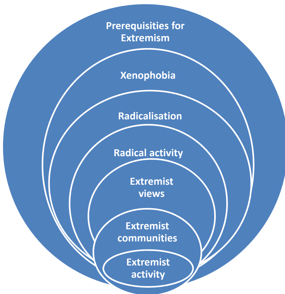
Diagram 1: Model for the Formation of Extremist Communities
