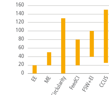
Figure 11.13 | Potentials and costs for zero-carbon mitigation options for industry and basic materials: CIEI – carbon intensity of electricity for indirect emissions; EE – energy efficiency; ME – material efficiency; Circularity – material flows (clinker substituted by coal fly ash, blast furnace slag or other by-products and waste, steel scrap, plastic recycling, etc.); FeedCI – feedstock carbon intensity (hydrogen, biomass, novel cement, natural clinker substitutes); FSW+EI – fuel switch and processes electrification with low-carbon electricity. Ranges for mitigation options are shown based on bottom-up studies for grouped technologies packages, not for single technologies. In circles, contribution to mitigation from technologies based on their readiness are shown for 2050 (2040) and 2070. Direct emissions include fuel combustion and process emissions. Indirect emissions include emissions attributed to consumed electricity and purchased heat. For basic chemicals only methanol, ammonia and high-value chemicals are considered. The total for industry doesn't include emissions from waste. Base values for 2020 for direct and indirect emissions were calculated using 2019 GHG emission data (Crippa et al. 2021) and data for materials production from World Steel Association (2020a) and IEA (2021d). Negative mitigation costs for some options like Circularity are not reflected. Data from sources: Pauliuk et al. (2013a); Fawkes et al. (2016); WBCSD (2016); Bazzanella and Ausfelder (2017); IEA (2018a, 2019b,g,h, 2020a,c, 2021a); Lehne and Preston (2018); Scrivener et al. (2018); EUROFER (2019); Friedmann et al. (2019); Material Economics (2019); Sandalow et al. (2019); CAT (2020); CEMBUREAU (2020); Gielen et al. (2020); Habert et al. (2020); World Steel Association (2020b); Bataille (2020a); GCCA (2021a); and Saygin and Gielen (2021).
