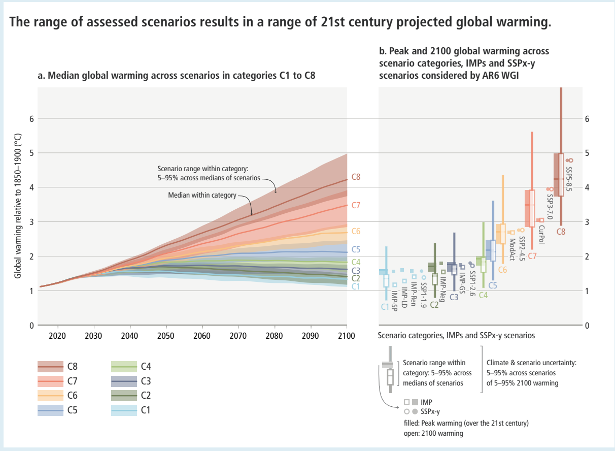
Box SPM.1, Figure 1 | Projected global mean warming of the ensemble of modelled scenarios included in the climate categories C1–C8 and IMPs (based on emulators calibrated to the WGI assessment), as well as five illustrative scenarios (SSPx-y) as considered by AR6 WGI. Panel a shows the p5–p95 range of projected median warming across global modelled pathways within a category, with the category medians (line). Panel b shows the peak and 2100 emulated temperature outcomes for the categories C1 to C8 and for IMPs, and the five illustrative scenarios (SSPx-y) as considered by AR6 WGI. The boxes show the p5–p95 range within each scenario category, as in panel a. The combined p5–p95 range across scenarios and the climate uncertainty for each category C1–C8 is also shown for 2100 warming (thin vertical lines). (Table SPM.2) {Figure 3.11; AR6 WGI Figure SPM.8}
